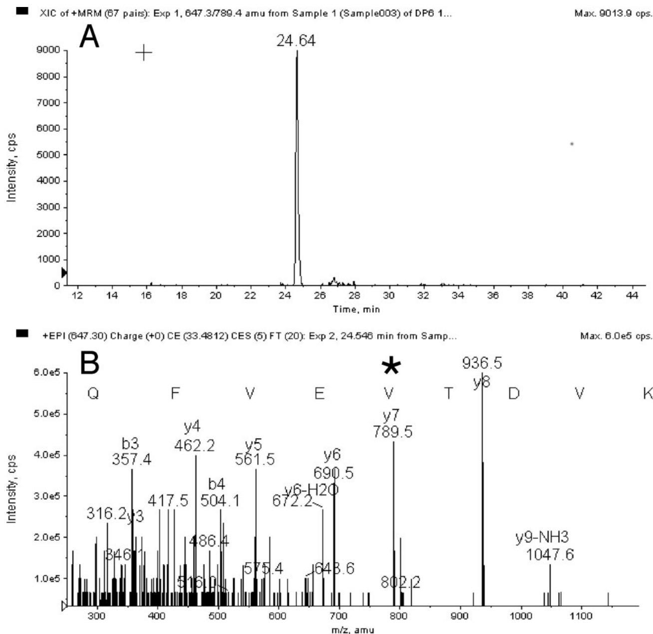
FIG. 1. MIDAS workflow (MRM-triggered MS/MS) verification of the identity of peptide DLQFVEVTDVK representing fibronectin (normal concentration, ~300 \mu\text{g/ml} ) in a digest of depleted human plasma. A shows the ion current profile of MRM 647.3/789.4 (MS1/MS2), and B shows the MS/MS spectrum of peptide fragments taken at the time of the peak (* marks the y7 fragment monitored in this MRM). cps, counts per second.
